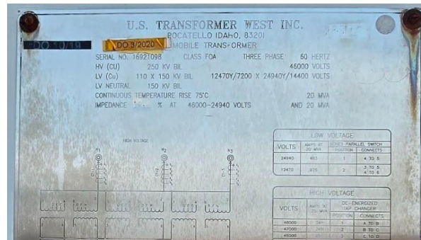
Main transformer nameplate · serial 16921098
